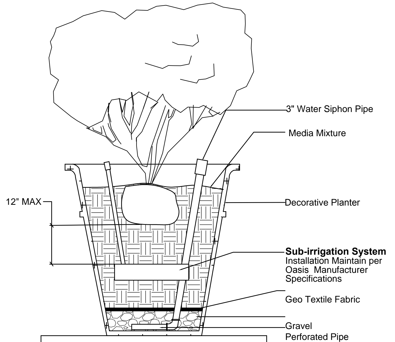
Single Tier Sub-Irrigation System
